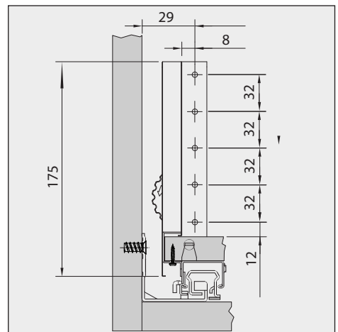
Implantation arrière Back drilling and installation
