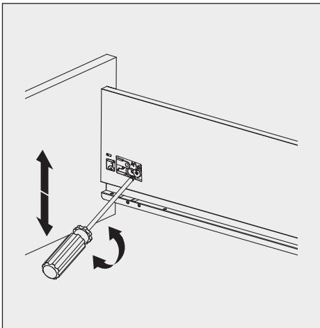
Réglage vertical \pm 2 mm Vertical adjustment \pm 2 mm
